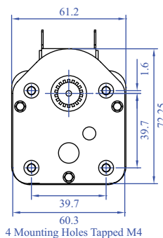
4 Mounting Holes Tapped M4
